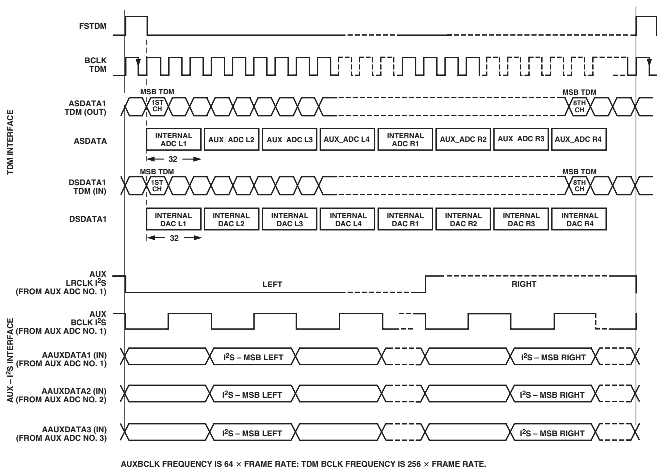
Figure 11. Auxiliary Mode Timing
