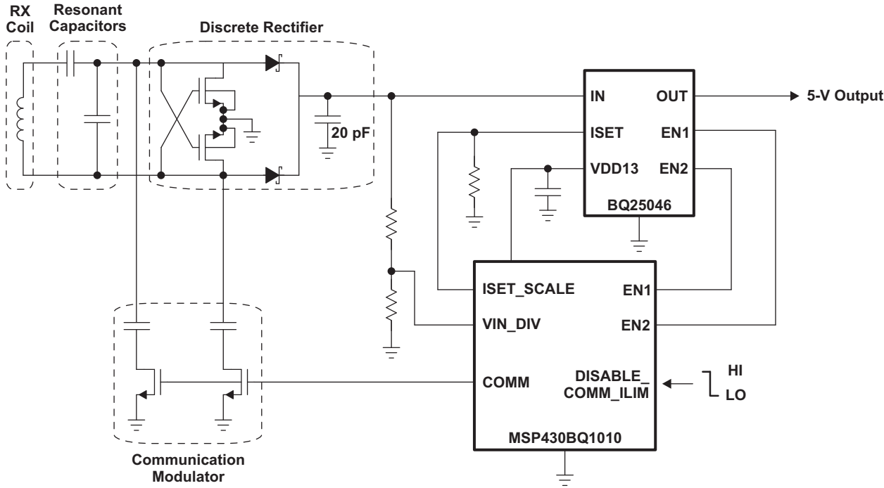
Figure 1. Application Schematic
