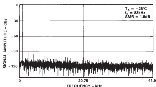
Figure 12. DAC FFT Plot
