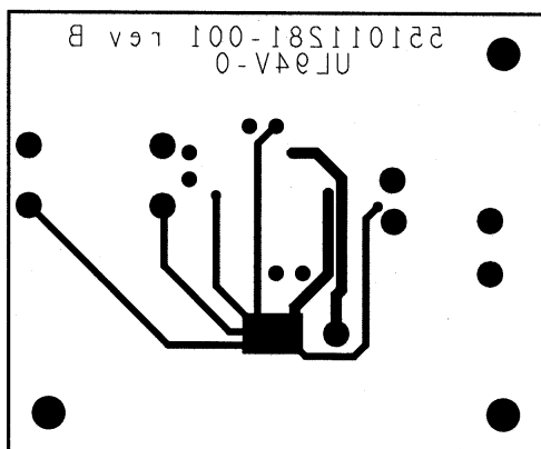
Figure 42. Bottom Layer
