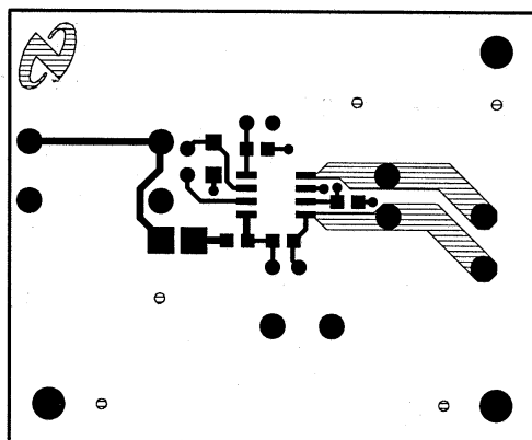
Figure 41. Top Layer
