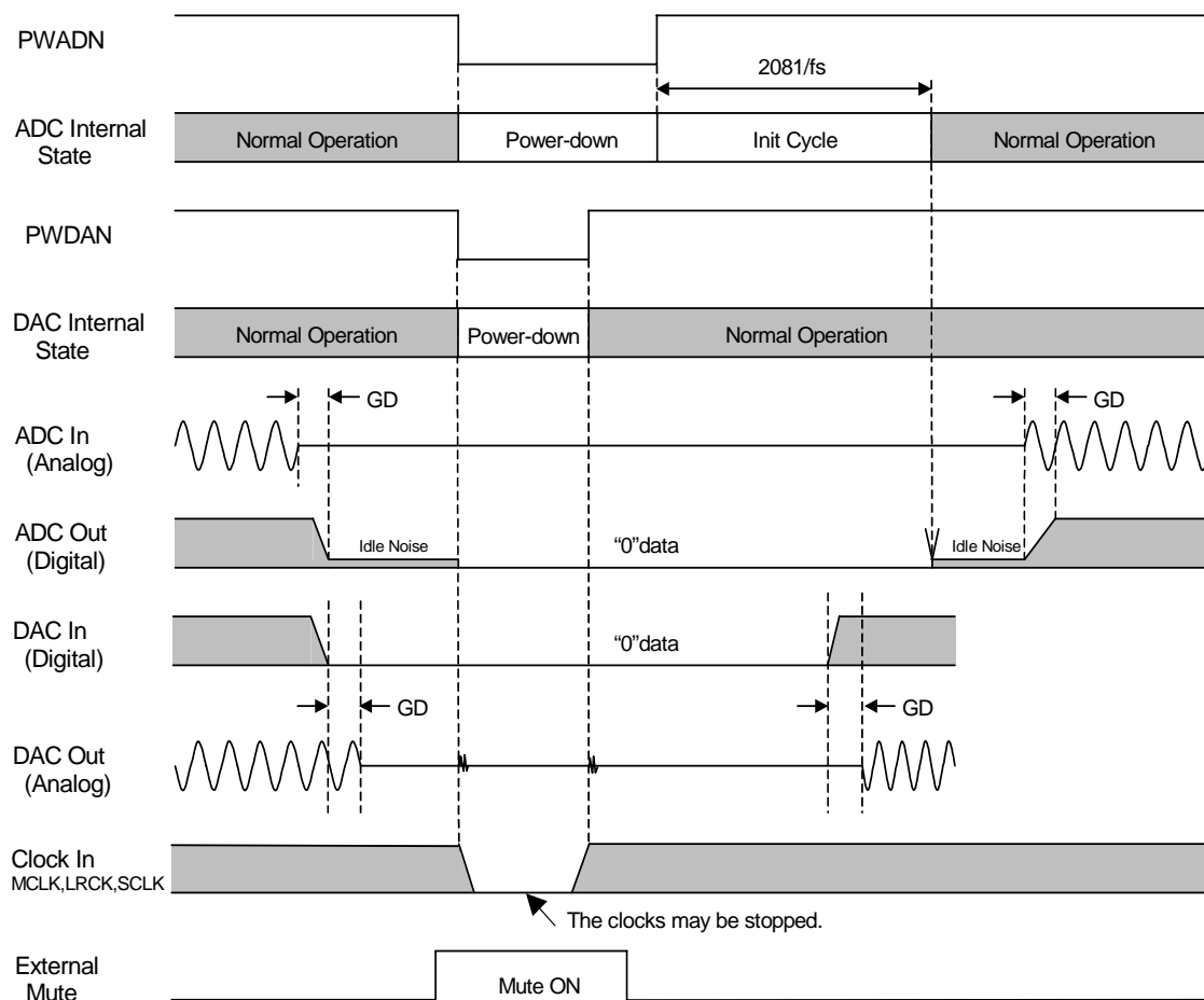
Figure 5. Power-up Sequence
