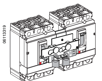
Interlocking with Toggle Control (S29354)
