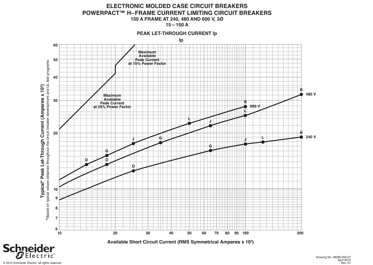
Figure 68: H-Frame 150 A Typical Peak Let-Through Curves
