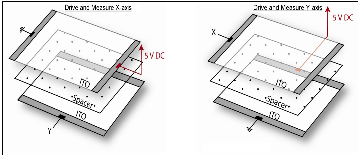
FIGURE 2-1: 4-WIRE DECODING
