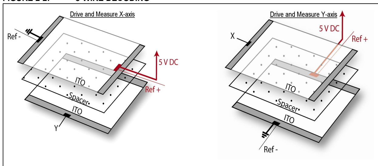
FIGURE 2-2: 8-WIRE DECODING
