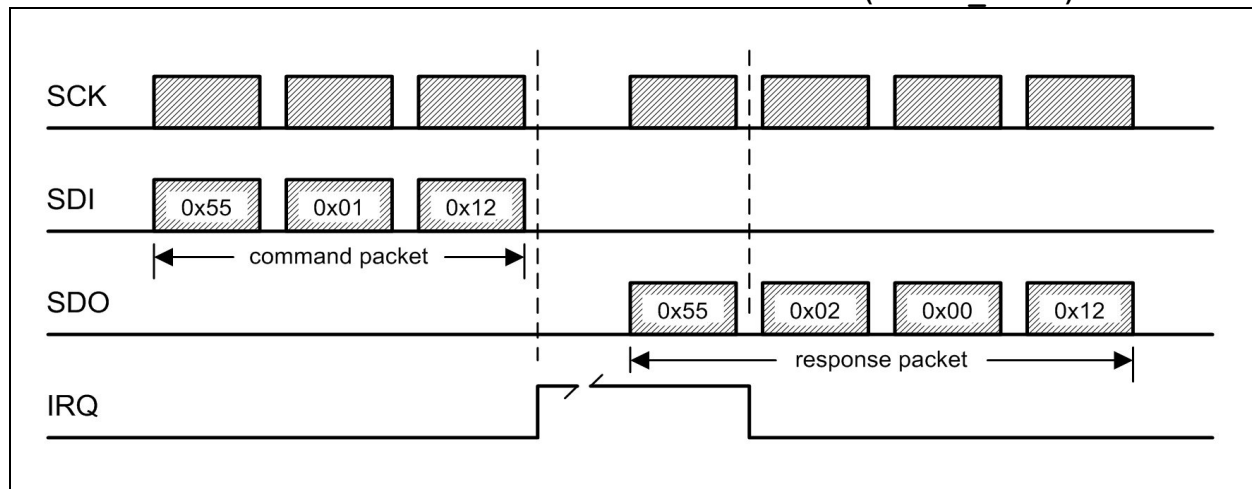
FIGURE 5-2: SPI TIMING DIAGRAM – COMMAND PROTOCOL ( ENABLE_TOUCH )
