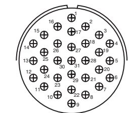
32-31 Service Rating A Number of Contacts 31 Contact Size 16
