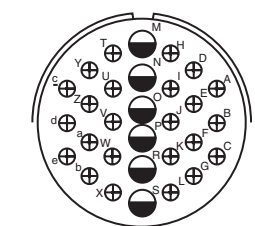
32-56 Service Rating A Number of Contacts 24 6 Contact Size 16 12 for #10 wire
