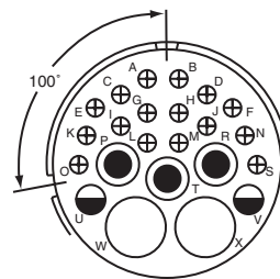
100° Rotation of 32-6 32-16 Service Rating A Number of Contacts 2 3 2 16 Contact Size 4 8 12 16
