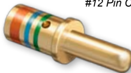
#12 Pin Contact
