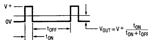
Figure 10. The LTC1040 as a Linear Amplifier
