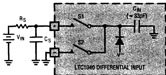
Figure 1. Equivalent Input Circuit
