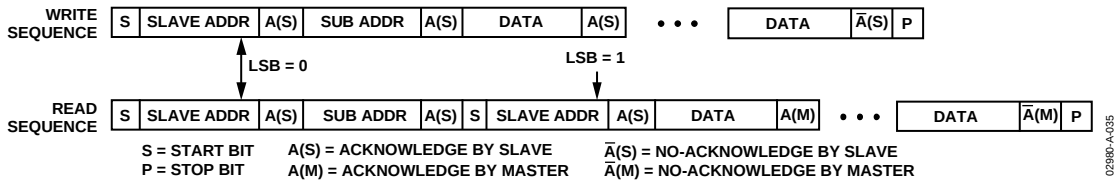
Figure 36. Write and Read Sequences
