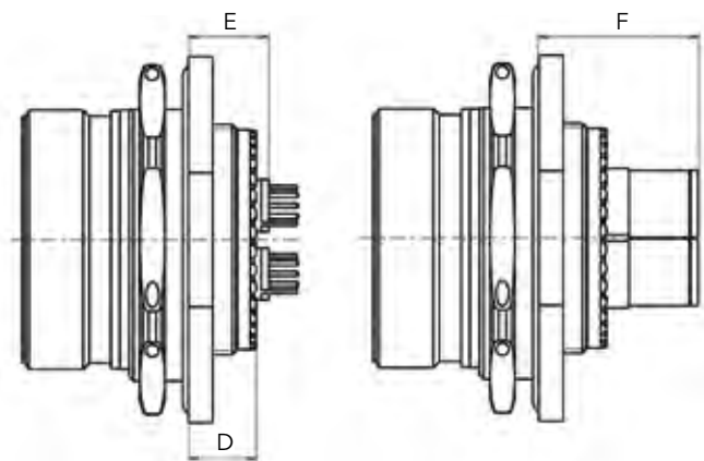
PC Tail contacts Crimp contacts
