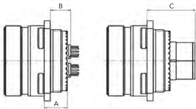
PC Tail contacts Crimp contacts
