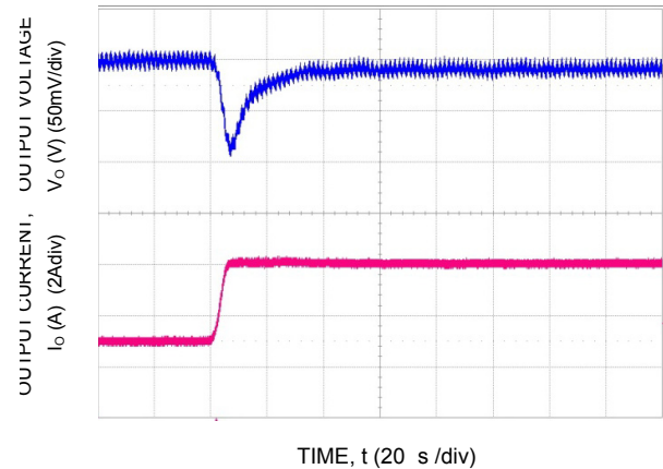
Figure 34. Transient Response to Dynamic Load Change from 50% to 100% at 12Vin, C_{Out}=2 \times 47\mu F , CTune-2200pF & RTune-261
