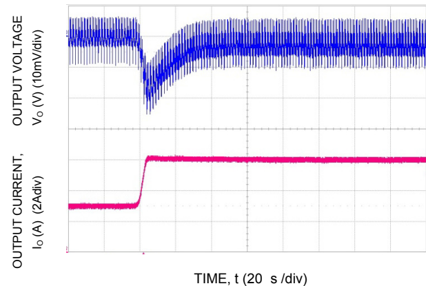
Figure 10. Transient Response to Dynamic Load Change from 50% to 100% at 12V in , C out -1x47 \mu\text{F} +3x330 \mu\text{F} , CTune-12nF & RTune-178
