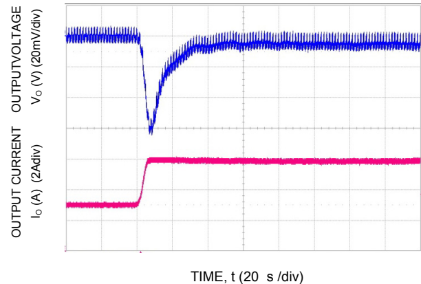
Figure 28. Transient Response to Dynamic Load Change from 50% to 100% at 12V in , C_{out}=3\times 47\mu\text{F} , CTune-178 & RTune-3900pF
