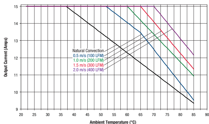
Maximum Current Temperature Derating @ sea level ( V_{in} = 48\text{ V} , transverse airflow, no baseplate)
