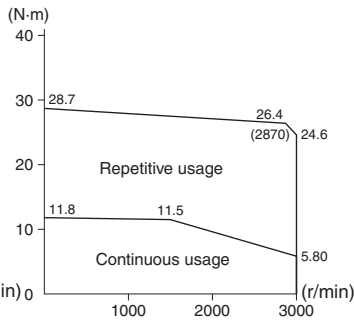
R88M-W7K515T (7.5 kW)
