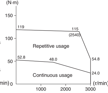
R88M-W7K515T (7.5 kW)
