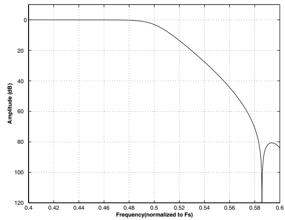
Figure 22. Double Speed (fast) Transition Band
