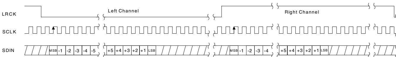
Figure 6. I 2 S, up to 24-Bit Data
