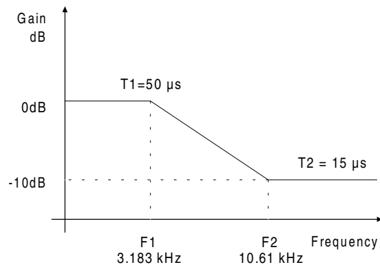
Figure 8. De-Emphasis Curve
