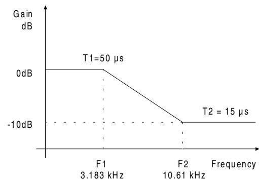
Figure 11. De-Emphasis Curve
