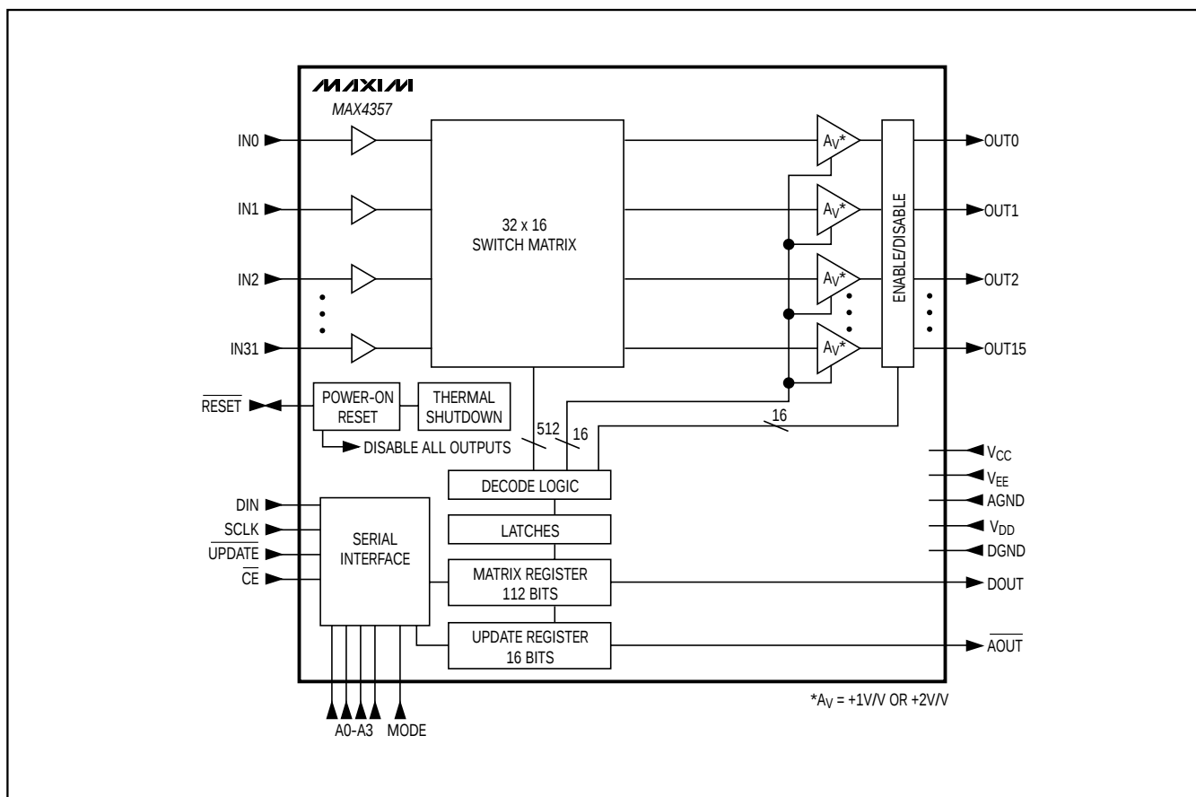
Functional Diagram
