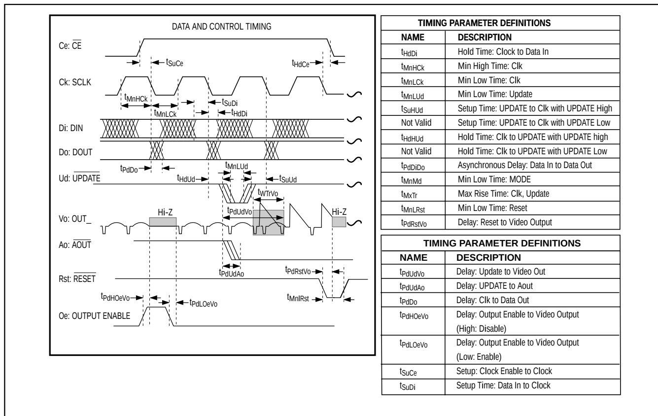
Figure 1. Timing Diagram
