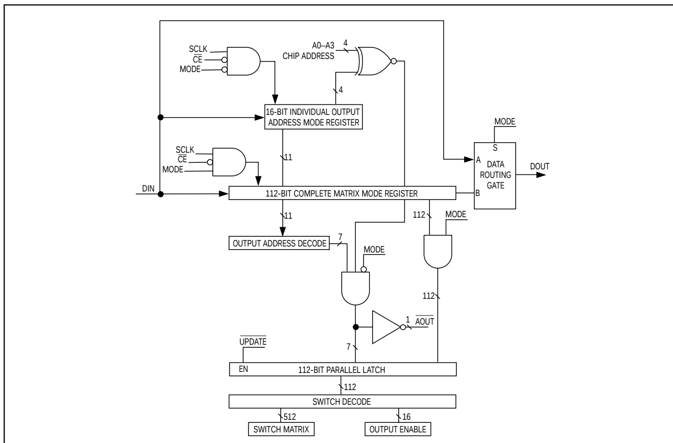
Figure 2. Serial Interface Block Diagram
