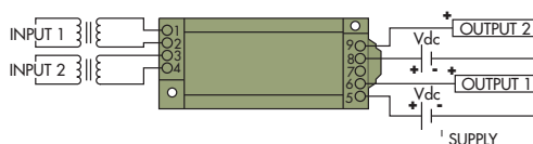
CR4640 Two Element with External Voltage Transformers **
