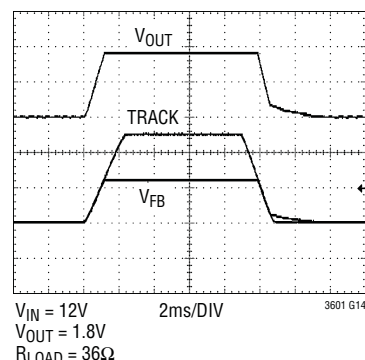
Output Tracking
