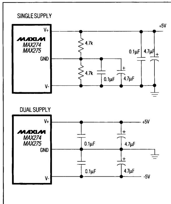
Figure 9. Power-Supply Configurations
