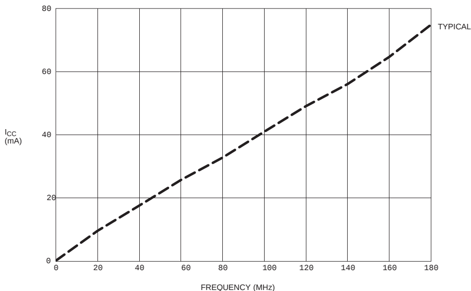
SP00442 Figure 4: I_{CC} vs Frequency (25°C)
