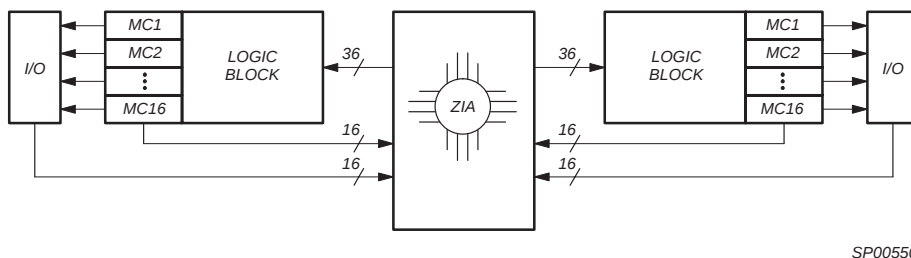
Figure 1: Xilinx XPLA CPLD Architecture
