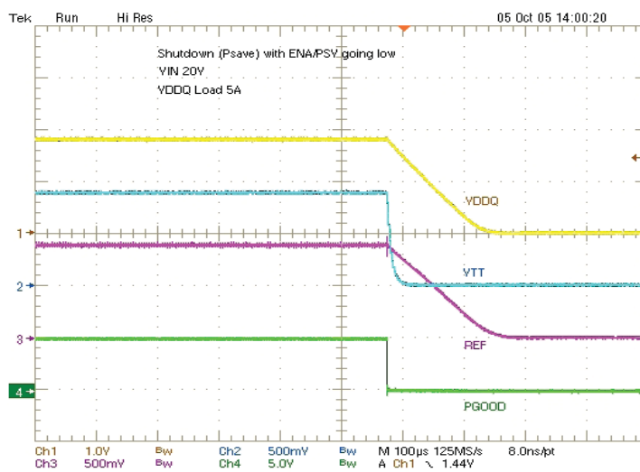
Startup (PSV), EN/PSV Going Low, VDDQ = 5A
