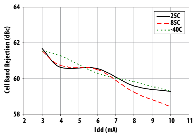
Figure 12. Cell band rejection vs. Idd at Vdd = 2.7V
