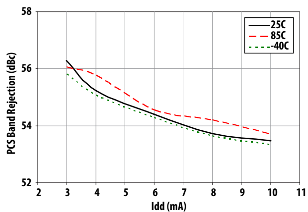
Figure 14. PCS band rejection vs. Idd at Vdd = 2.7V
