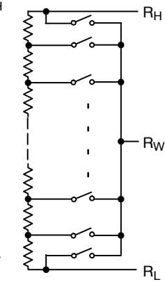
Figure 3. Electronic Potentiometer Implementation
