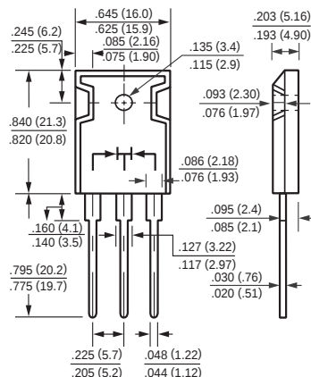
TO-247
