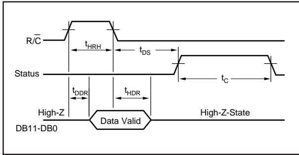
FIGURE 4. R/ \bar{C} Pulse High — Outputs Enabled Only While R/ \bar{C} Is High.
