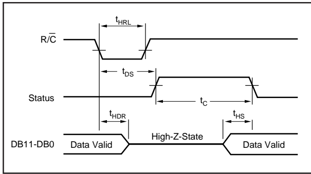
FIGURE 3. R/ \bar{C} Pulse Low—Outputs Enabled After Conversion.
