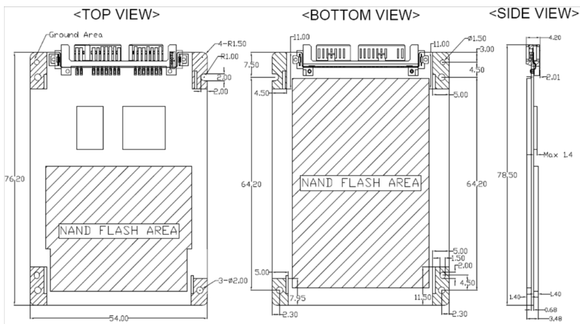
Figure 2-1. Physical dimension
