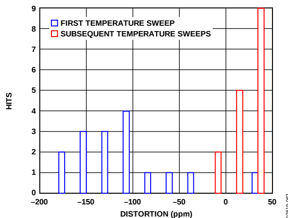
Figure 48. Thermal Hysteresis
