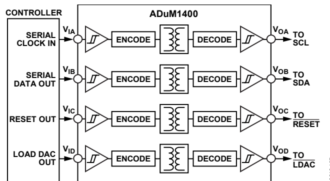
Figure 51. Isolated Interface
