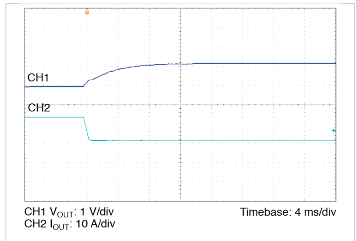
Figure 7 — 100% to 10% load transient response, V_{IN} = 28\text{ V} , nominal trim, C_{OUT\_EXT} = 250\text{ }\mu\text{F}
