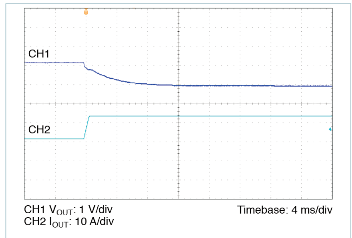
Figure 8 — 10% to 100% load transient response, V_{IN} = 28\text{ V} , nominal trim, C_{OUT\_EXT} = 250\text{ }\mu\text{F}
