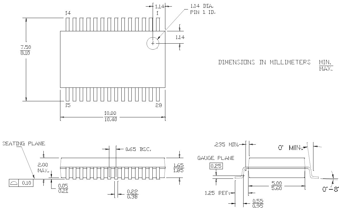
Figure 23-4. 28-Pin (5.3 mm) Shrunk Small Outline Package O28
