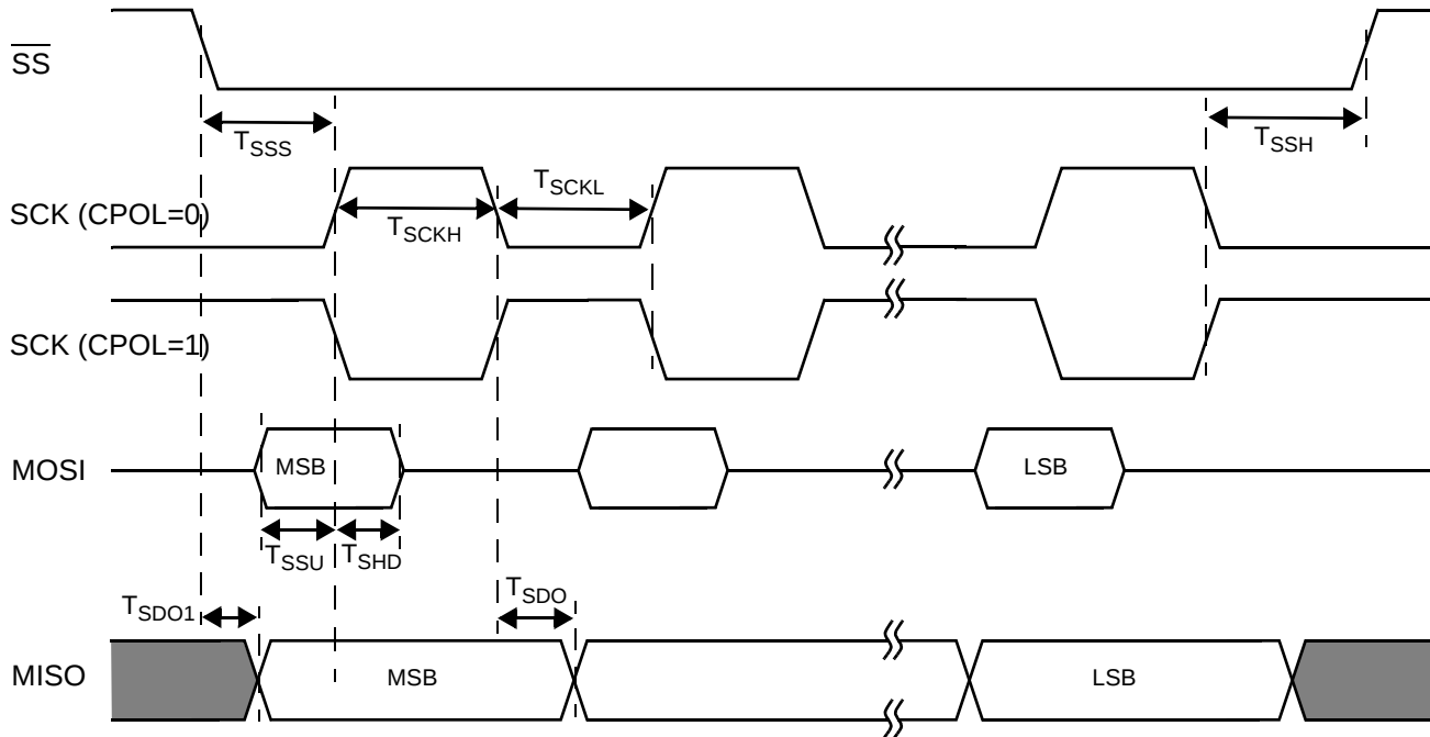
Figure 20-6. SPI Slave Timing, CPHA = 0
