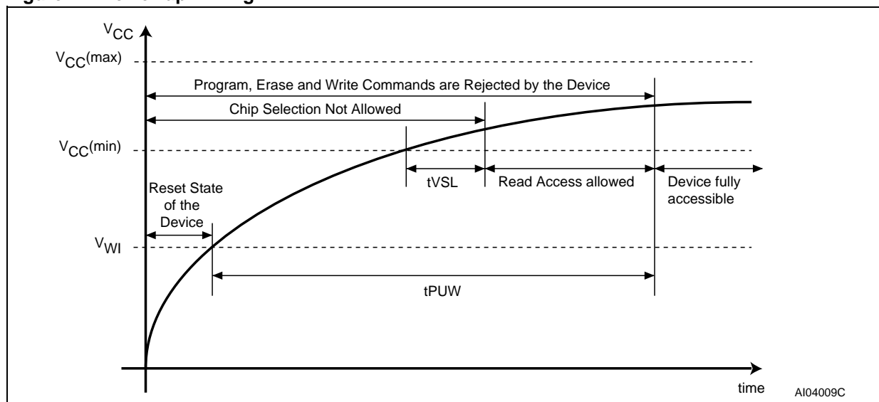
Figure 22. Power-up Timing
