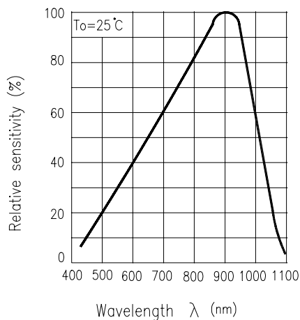
Fig.3 Spectral Sensitivity
