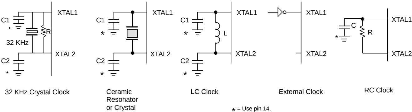
Figure 15. Oscillator Configuration
