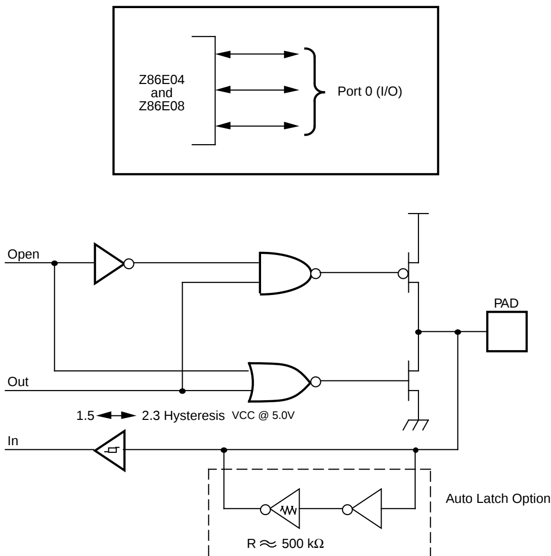
Figure 6. Port 0 Configuration
