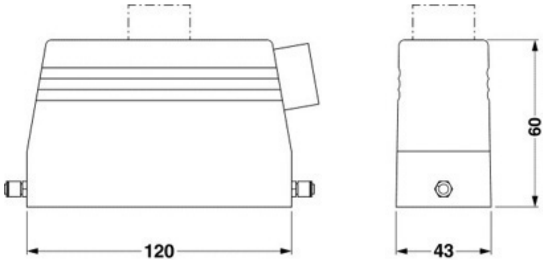
Dimensioned drawing
