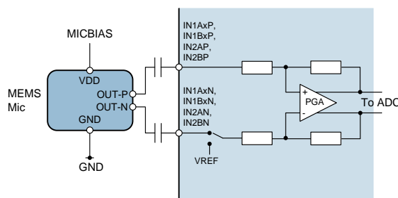
Figure 14 Differential MEMS Input
