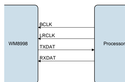
Figure 39 Slave Mode
