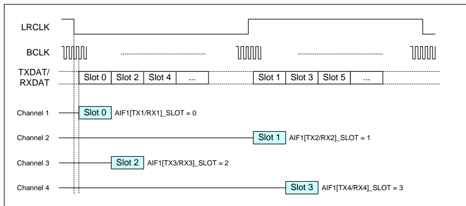
Figure 46 I2S Example
