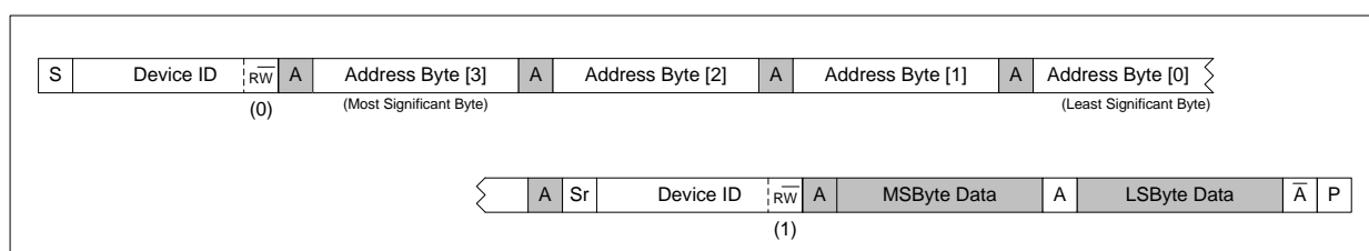
Figure 70 Single Register Read from Specified Address
