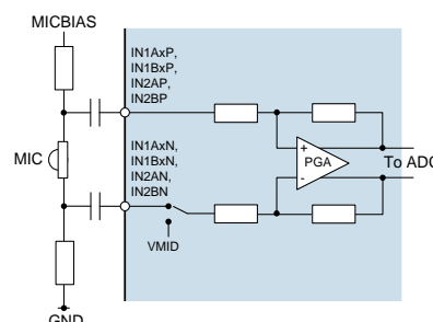
Figure 12 Differential ECM Input
