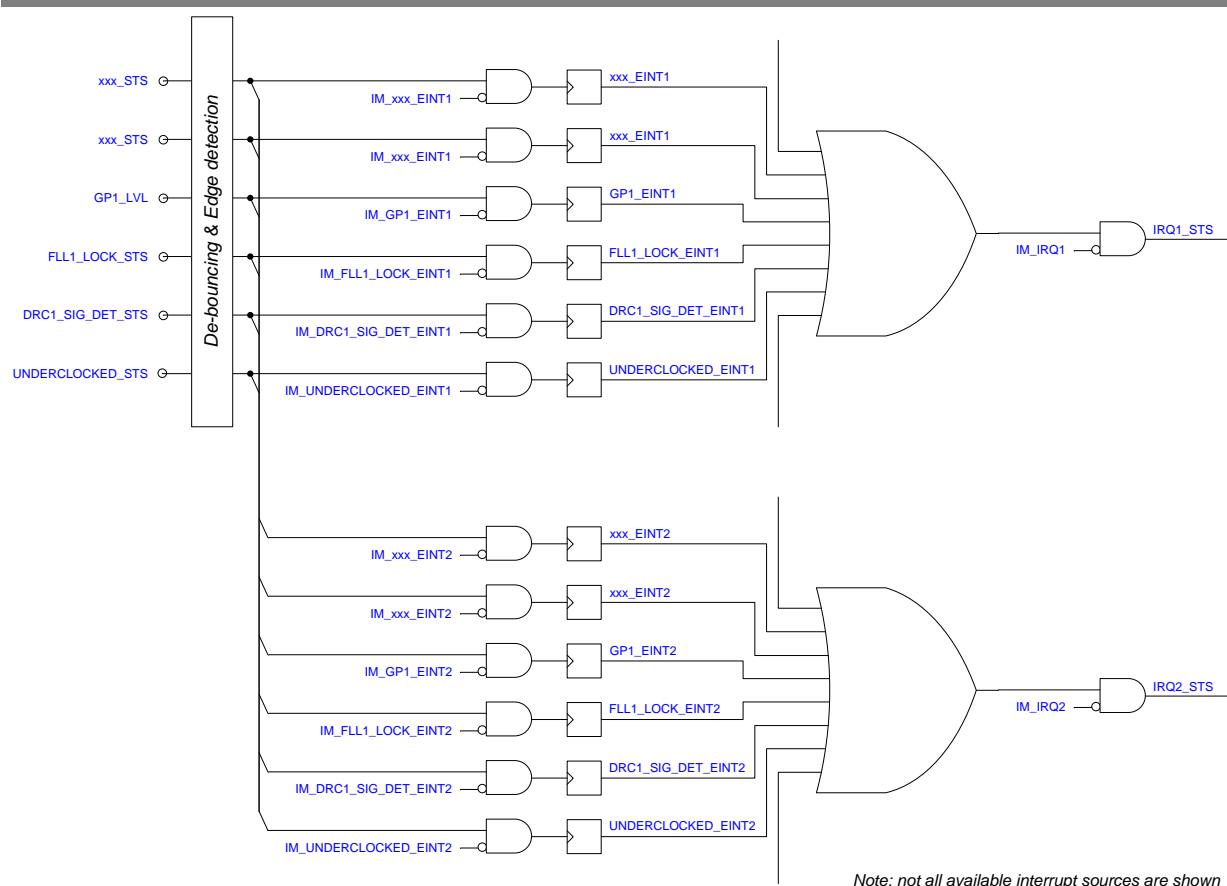
Figure 63 Interrupt Controller
