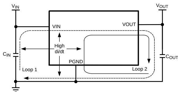
Figure 56. Critical Current Loops to Minimize
