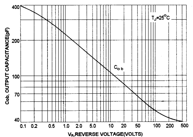
OUTPUT CAPACITANCES
