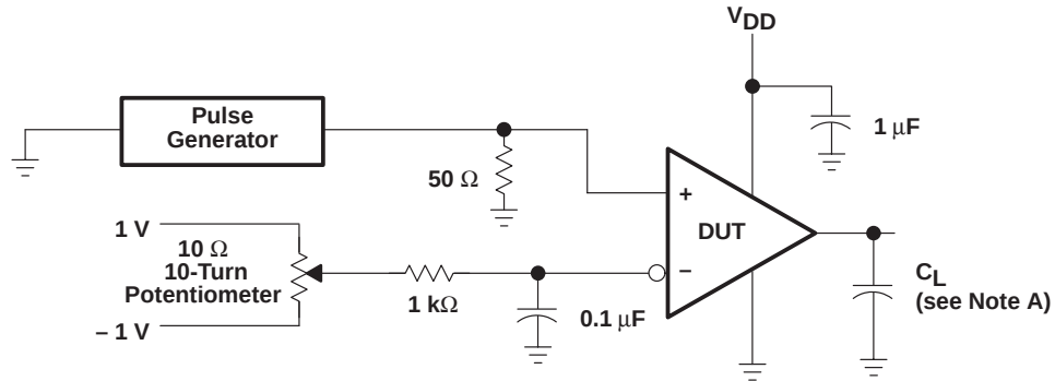
TEST CIRCUIT
