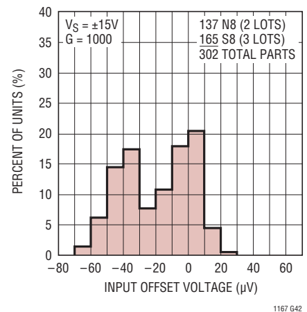
Distribution of Input Offset Voltage, T_A = 85^\circ\text{C}
