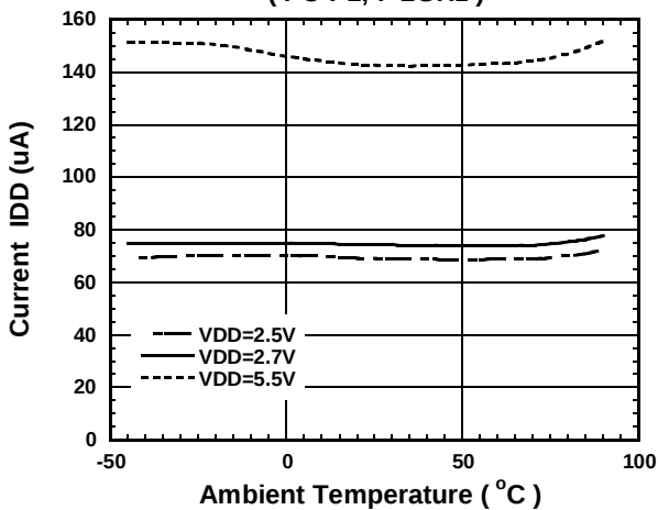
Current IDD vs. Ambient Temperature
