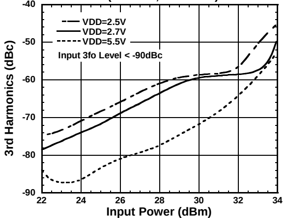
3rd Harmonics vs.Input Power ( f=2GHz, PC-P1on )
