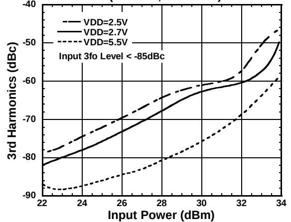
3rd Harmonics vs.Input Power ( f=1GHz, PC-P1on )
