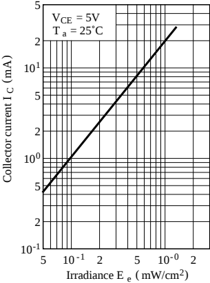
Fig.4-b Collector Current vs. Irradiance (PT550F)
