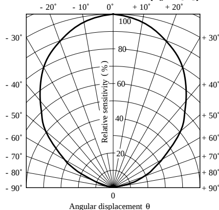
Fig.8-b Sensitivity Diagram (PT550F) ( T_a = 25^\circ\text{C} )
