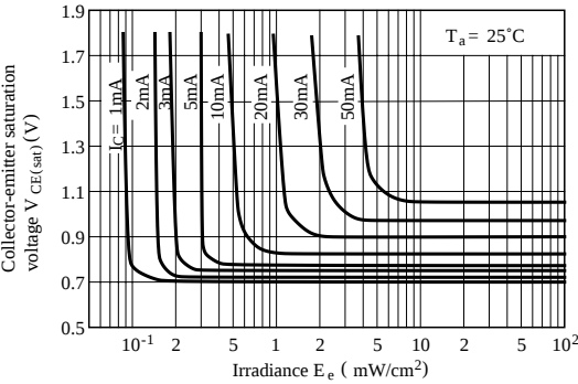
Fig.9-b Collector-emitter Saturation Voltage vs. Irradiance (PT550F)
