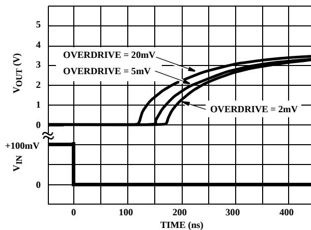
FIGURE 7. RESPONSE TIME FOR VARIOUS INPUT OVERDRIVES
