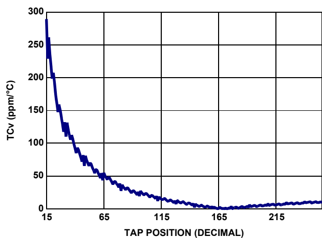
FIGURE 13. 10k TCv vs TAP POSITION
