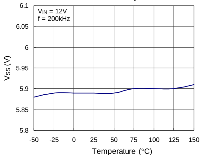
Soft Start vs. Temperature
