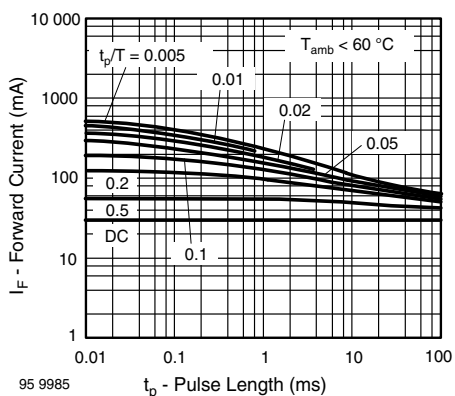
Fig. 2 - Permissible Pulse Forward Current vs. Pulse Duration
