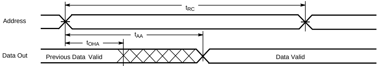
Figure 6. Read Cycle No. 2 (Either Port \overline{\text{CE}}/\overline{\text{OE}} Access) [13, 15, 16]
