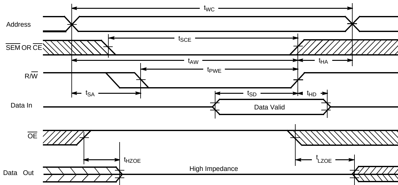
Figure 9. Write Cycle No. 2: \overline{\text{R/W}} Three-State Data I/Os (Either Port) [19, 21, 22]
