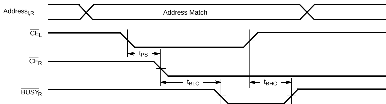
Figure 14. Busy Timing Diagram No. 1 ( \overline{CE} Arbitration) [28]
