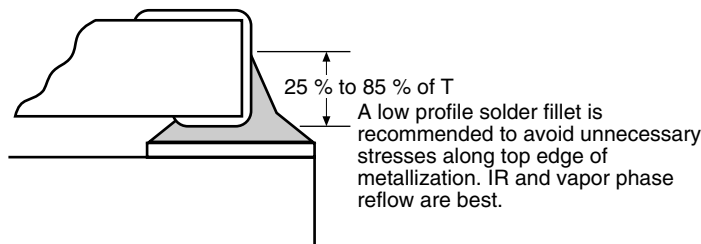
FIGURE 4 - RECOMMENDED MOUNTING (1)(2)(3)
