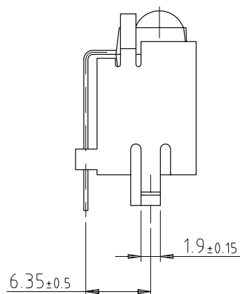
View "A"
