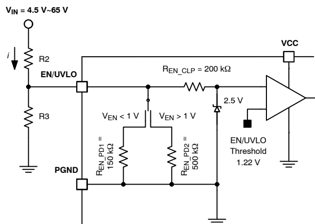
Figure 40. EN/UVLO Block Diagram
