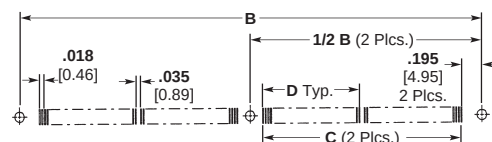
Recommended PCB Footprint Pattern
